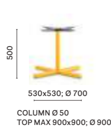
4758 H500 Coffee table base, cast-iron base
