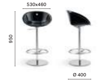
975 Barstool, polycarbonate shell, stainless steel central base
