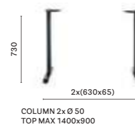
4757 Dining table base, cast-iron base
