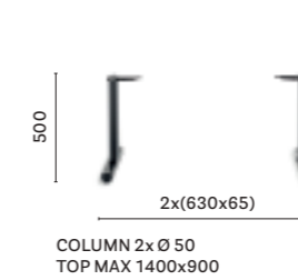
4757 H500 Coffee table base, cast-iron base
