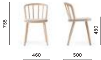
2840 Ash wood side chair with trestle legs
